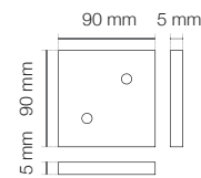
TAPA PILAR DIAMOND FENCE 90 mm x 90 mm
