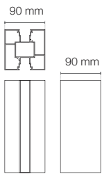
PILAR ALUMINIO DIAMOND FENCE 90 mm x 90 mm
